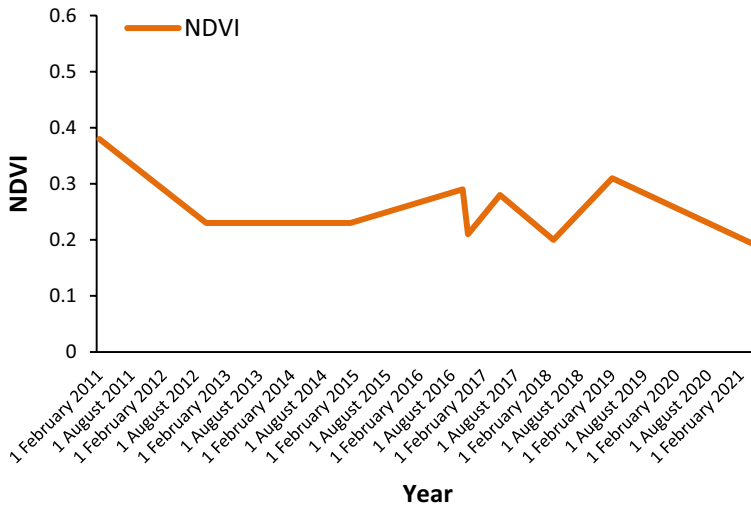
Fig. 9 NDVI results for Bands 3 and 4 in Kolar district
