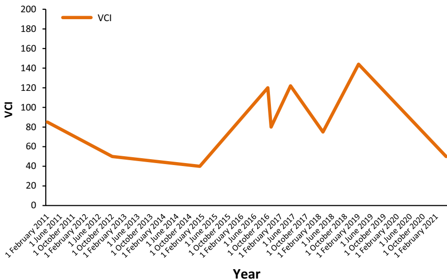
Fig. 10 VCI values for Band 3 and Band 4
